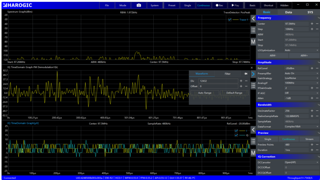
Figure 32 FM demodulation analysis in IQS mode.
